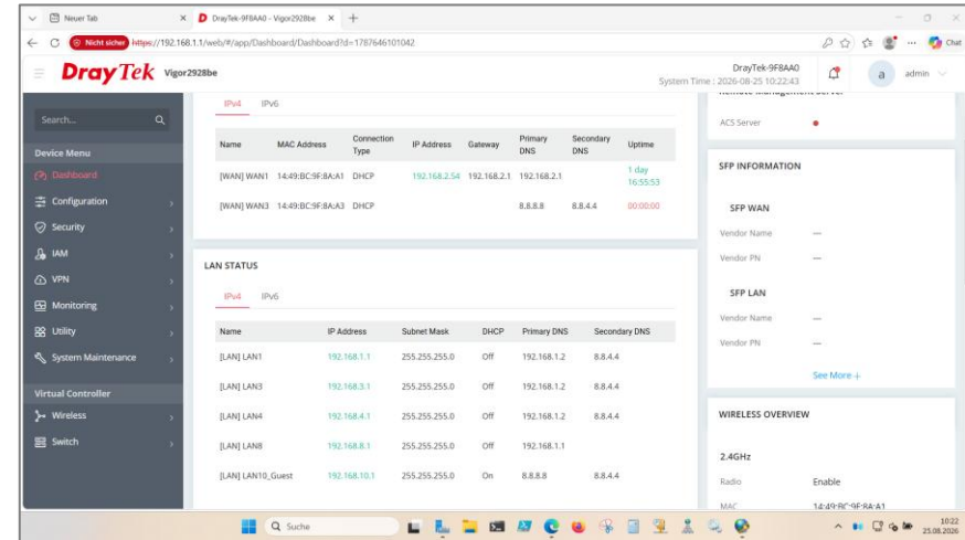
Dashboard | LAN Status IPv4 | LAN10_Guest
